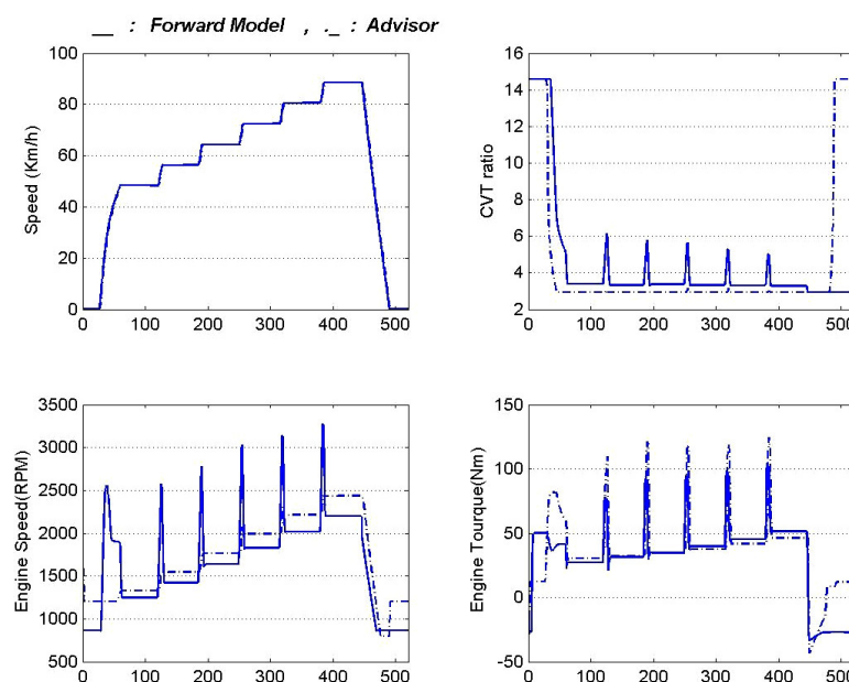
Fig. 14. Results for second pedal cycle.
