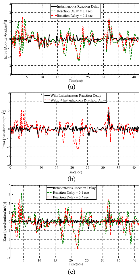
Fig. 12. estimation error for car-following models: (a) ANN, (b) FIS, (c) ANFIS.
