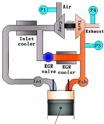
Fig4. EGR architecture
