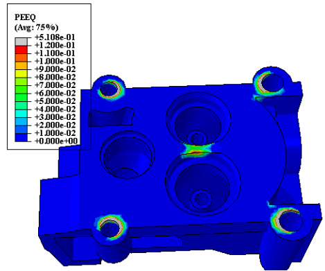
Fig10. The equivalent plastic strain distribution.
