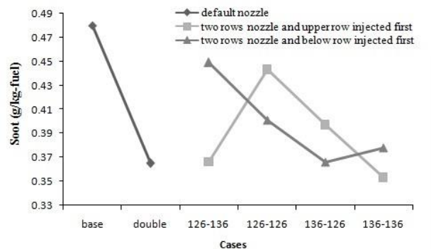
Fig 13. Soot emission
