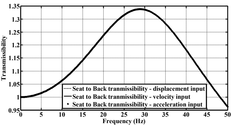
Fig31. Seat to back transmissibility
