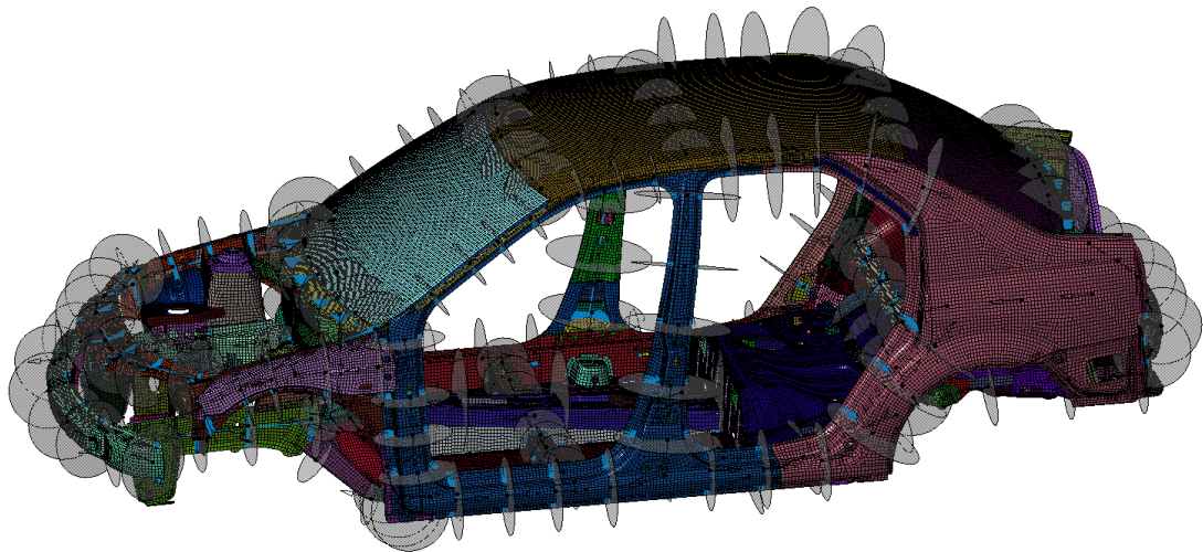
Fig2.: Sections defined on the beams to simplify the BIW
