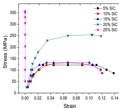
Figure 2: Stress – Strain Curve for varying %wt Silicon-Carbide
