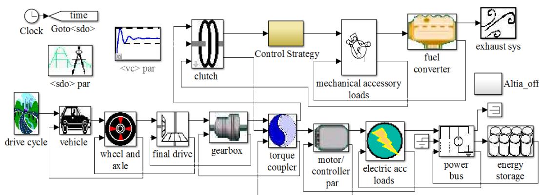
Figure 4: Model of the PHEV
