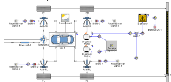
Figure 6. Modified vehicle model with in wheel motors and batteries
