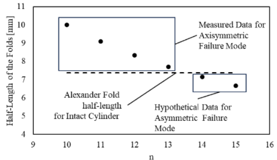
Figure 27: Axisymmetric half-length of fold for ST perforated cylinders (H).
