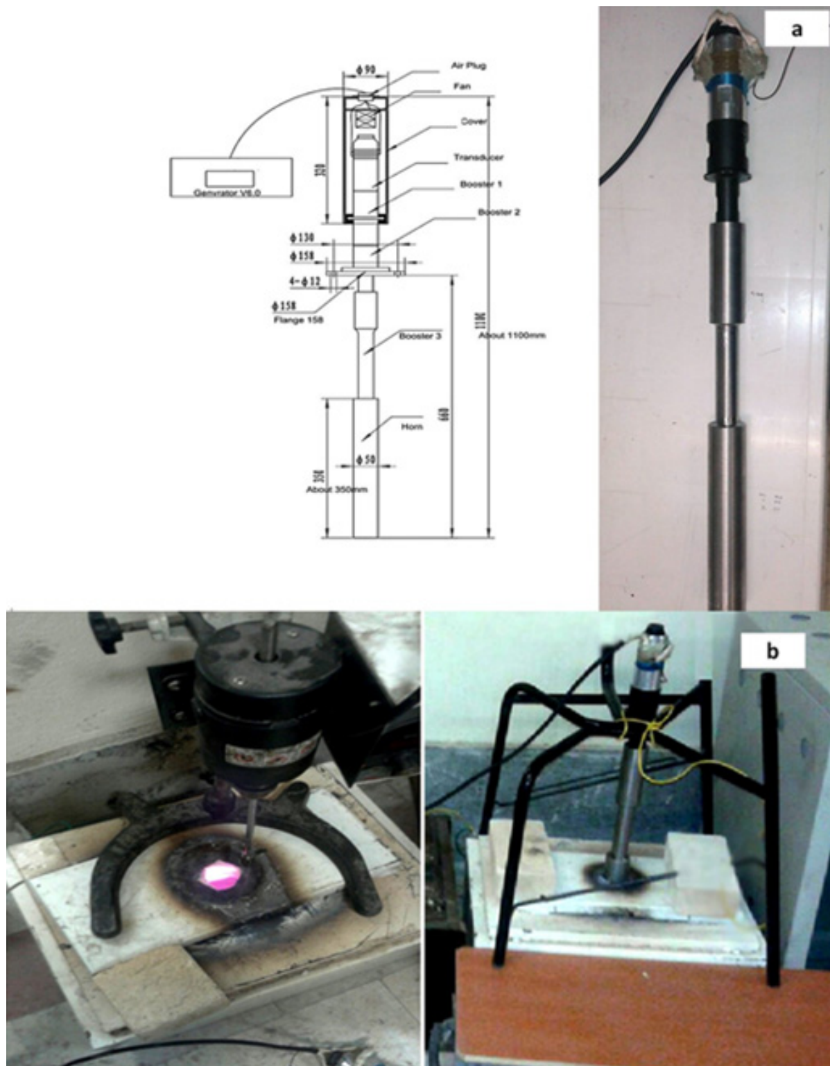
Fig. 4. a) Ultrasonic probe and (b) mechanical stirrer and ultrasonic device.
