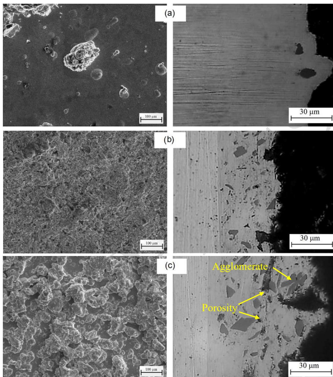
Figure 2. SEM micrographs of top surface and cross-section of composite coatings electro-deposited by PRC with different concentrations of a) 5, b) 10, and c) 15 g/l B 4 C micro particles in electroplating bath
