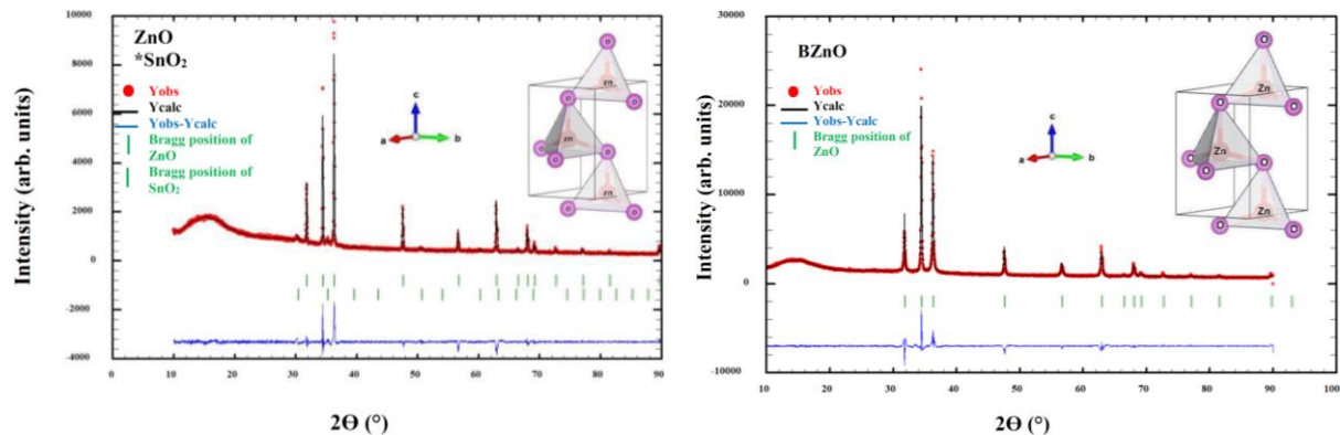
Fig. 2. Rietveld refined X-ray diffraction patterns for ZnO and BZnO microrod samples. Observed (calculated) profiles are shown by dotted (solid lines). The short vertical marks represent Bragg reflection. The lower curve is the difference plot. The inset presents the hexagonal structure of ZnO and BZnO microrods
