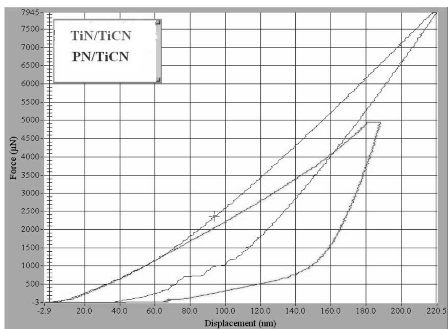
Fig.6. load-displacement curves.
