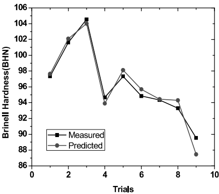
Fig. 8. Comparison plots of the measured and predicted hardness of 6061 Aluminium alloy
