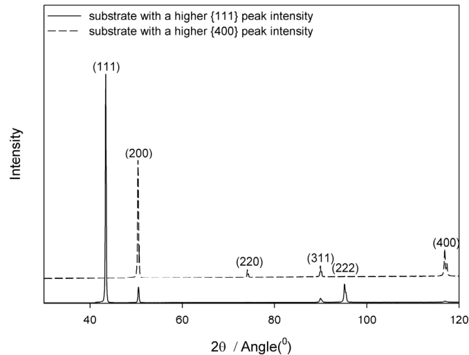
Fig. 1. XRD peak profiles of the copper substrates with two different grain orientations.
