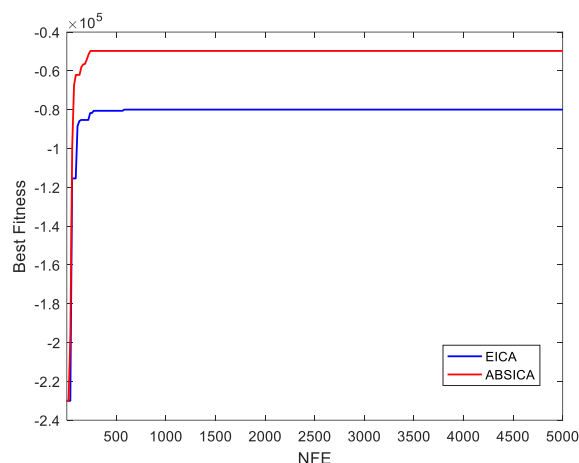
Figure 4. Convergence curves for the best results of 928-bar design problem
